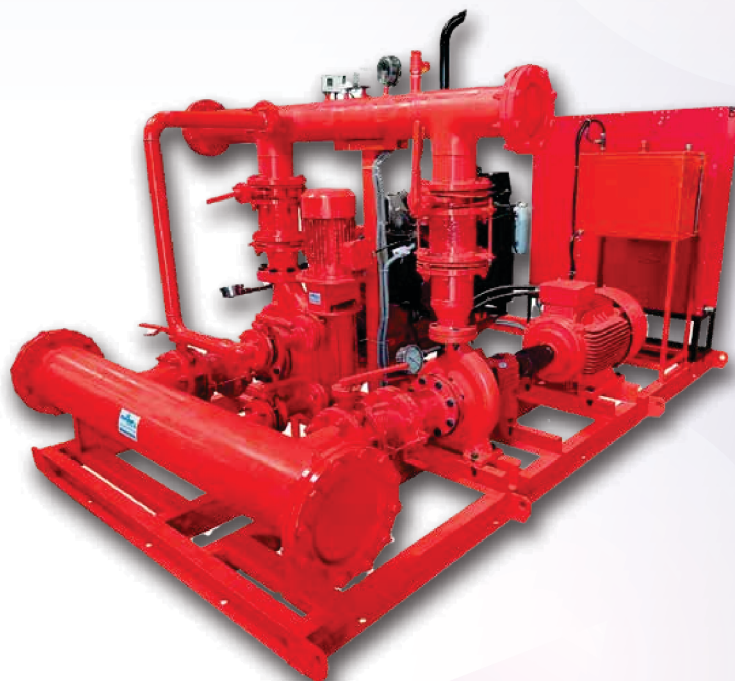
FIRE FIGHTING SKID MOUNTING SYSTEM
